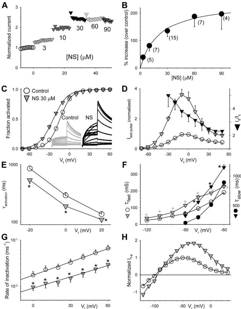
Fig. 2. Characterization of the effects of NS on the hERG channel expressed in oocytes. Voltage clamp protocols and methods of data analysis are the same as those described for corresponding panels in Fig. 1. [NS] for experiments shown in C to H was 30 \mu\text{M} . A, time course of changes in hERG current amplitude before and during exposure to NS at the specified concentrations. B, concentration-response relationship. The superimposed curve was calculated from the equation I_d/I_c = 1 + (A - 1)/(1 + K_d/[D]) with A (fold increase in current amplitude) = 3.24 and K_d = 20 \mu\text{M} . C, NS shifted the 1-s isochronal activation curve of hERG in the negative direction by -9.8 \pm 1.4 \text{ mV} ( n = 7 ). D, NS increased hERG test pulse current in a voltage-dependent manner. E, NS accelerated hERG activation (shortened \tau_{\text{activation}} ). F, NS slowed hERG deactivation, manifested as a prolongation of \tau_{\text{fast}} and \tau_{\text{slow}} . G, NS slowed hERG inactivation. The lines superimposed on the data points were calculated from K(V_t) = K(0)\exp(z_{\text{ina}}V_tF/RT) (described for Fig. 1G), with values of K(0) and z_{\text{ina}} of 0.02 \text{ms}^{-1} and 0.6 for control and 0.01 \text{ms}^{-1} and 0.5 for PD, respectively. H, NS increased both outward and inward currents through the hERG channel. * p < 0.05 , NS versus control.
