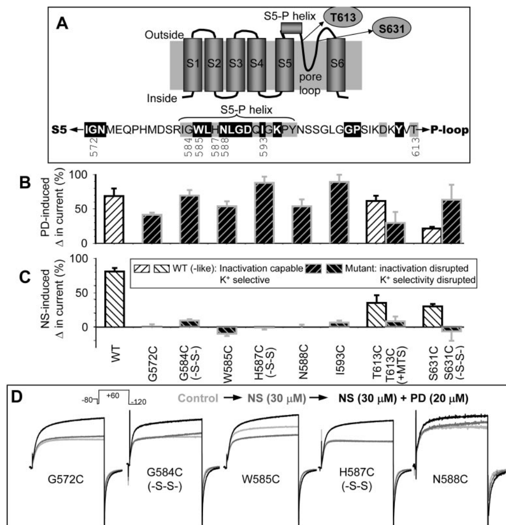
Fig. 6. Summary of effects of Cys substitution or Cys side chain modification introduced into the outer vestibule or pore entrance of the hERG channel on the activator action of PD307243 and NS1643. A , top, two-dimensional diagram of a hERG subunit, marking S1 to S6 transmembrane helices, pore loop, and the extracellular S5-P helix. Bottom, amino acid sequence of the S5-P linker, marking the positions that participate in forming the S5-P helix. High- and intermediate-impact positions are highlighted by white lettering on black shade and by gray shade, respectively. The positions examined in Figs. 6 and 7 are noted below the sequence. Thr613 and Ser631 are marked in the two-dimensional diagram. B and C , percentage change in current amplitude measured at 0 mV (WT or WT-like) or +60 mV (mutant) induced by 20 \mu\text{M} PD or 30 \mu\text{M} NS plotted against the channel types along the abscissa in C , where Cys side chains modified by disulfide bonding (-S-S-) or MTSET modification (+MTS) are noted. Hatched histogram bars for WT or WT-like channel phenotype are shown in white background, whereas those for mutant phenotype are shown in black background ( C , inset). D , superimposed current traces recorded from oocytes expressing the specified hERG mutants. Currents were elicited by the voltage clamp protocol diagrammed on top under three conditions: control (light gray traces), after adding 30 \mu\text{M} NS (dark gray traces), and after adding 20 \mu\text{M} PD in the continuous presence of NS (black traces).
