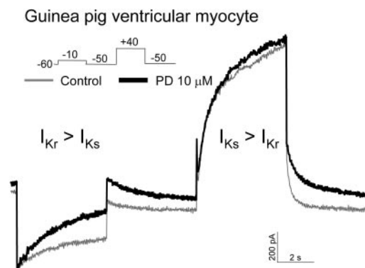
Fig. 10. Agonist effect of PD307243 on native I_{Kr} in a guinea pig ventricular myocyte. Shown are superimposed current traces recorded from the same myocyte before (thin gray trace) and 5 min after application of PD 10 \mu M (thick black trace). Currents were elicited by the pulse protocol diagrammed. Based on the difference in voltage-dependence of activation (Sanguinetti and Jurkiewicz, 1990), time-dependent current during the -10 mV step and the following tail current at -50 mV mainly represented I_{Kr} . Time-dependent current during the +50 mV step mainly represented I_{Ks} , although the following tail current resulted from both I_{Kr} and I_{Ks} .
