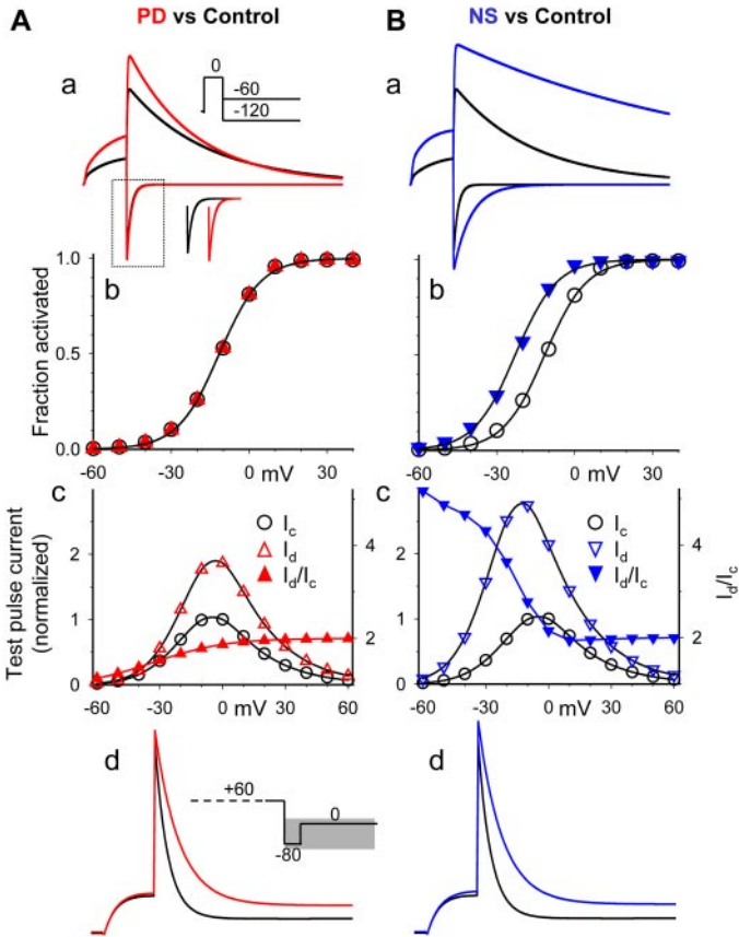
Fig. 3. Model simulation of the effects of PD307243 (A) and NS1643 (B) on the hERG channel. The model and parameter values are listed in Table 1. Simulated current traces and data points for control, PD and NS are shown in black, red and blue, respectively. For each column, a and d show superimposed simulated current traces elicited by the voltage clamp protocols diagrammed in the insets (time scale was the same as protocols shown in Fig. 1), b depicts simulated 1-s isochronal activation curves, and c illustrates simulated test pulse current-voltage relationship (open symbols, left coordinate) and current ratio (I d /I c , right coordinate). Inset of A, a, shows horizontally shifted inward tail currents at -120 mV, to illustrate the difference in the peak current amplitude.
