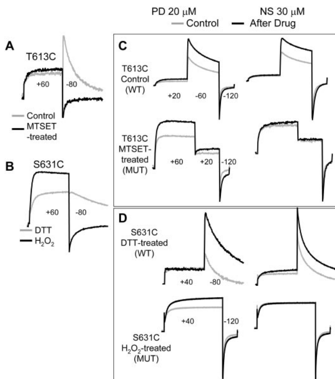
Fig. 7. Modifications of Cys side chains introduced into 2 pore entrance positions differentially affected the “activator” effects of PD307243 and NS1643. Currents were elicited by different voltage clamp protocols to 1) illustrate their gating behavior as WT-like or mutant and 2) probe for drug effects on both outward and inward currents through the channels. For the sake of simplicity, individual voltage-clamp protocols are not shown; only the step voltages are noted (holding voltage was -80 mV in all cases). A, T613C manifested WT-like gating behavior under the control conditions (gray trace), and switched to the mutant behavior after MTSET modification (black trace). B, S631C manifested WT-like behavior (gray trace) when DTT treated, but switched to mutant behavior (black trace) after H_2O_2 treatment with pulsing. C and D, PD was effective in increasing currents through the T613C and S631C channels in both WT-like and mutant behavior. On the other hand, NS was effective in increasing currents through the T613C and S631C channels in the WT-like mode but incapable of increasing currents when the channels were in the mutant mode.
