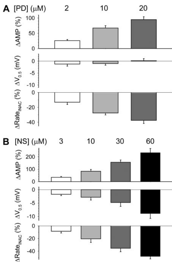
Fig. 4. Concentration-response relationships of PD307243 (A) and NS1643 (B) on hERG current amplitude and gating kinetics. \Delta\text{AMP} , percentage increase in current amplitude measured as time-dependent current during 1-s step to 0 mV; \Delta V_{0.5} , shift in V_{0.5} of activation; \Delta\text{Rate}_{\text{INAC}} , percentage decrease in rate of channel inactivation at 0 mV. Data were averaged from four to six measurements each.
