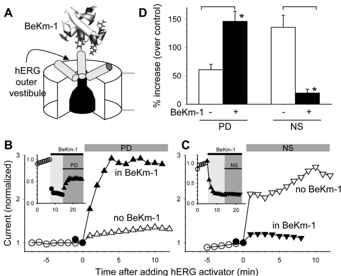
Fig. 8. BeKm-1 potentiated the activator effect of PD307243 but suppressed the activator effect of NS1643. A , cartoon of hERG pore domain with an extracellular BeKm-1 structure. Three hERG subunits are depicted, with the fourth one closest to viewers removed to reveal the narrow selectivity filter and wide inner cavity of the pore. Cylinders represent the S5-P helices. B , main plot, two time courses of changes in hERG current amplitude before and after exposure to 20 \mu M PD. Current amplitudes were measured from time-dependent currents during 1-s steps to 0 mV and normalized by the current right before PD application. One experiment (open symbols) was conducted in the absence of BeKm-1. The other (black symbols) was conducted in the presence of 10 \mu M BeKm-1. Inset, the complete time course of the second experiment. BeKm-1 suppressed the current by 80% and subsequent application of PD in the continuous presence of BeKm-1 effectively increased the current amplitude. C , NS (30 \mu M) effect on hERG in the absence or presence of BeKm-1. The format is the same as that of B . D , data summary. *, p < 0.05 , data obtained in the presence of BeKm-1 versus those without BeKm-1.
