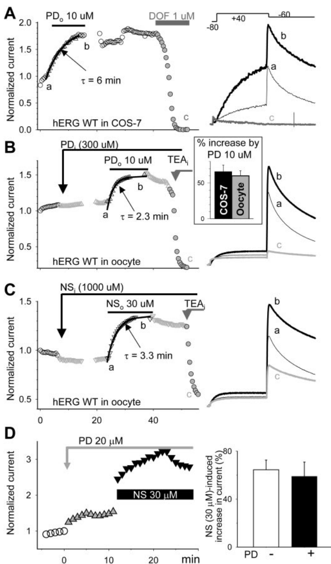
Fig. 5. Both PD307243 and NS1643 worked from outside the cell membrane, yet their effects were independent of each other. A , left, time course of changes in hERG current amplitude expressed in a COS-7 cell before, during, and after bath application of PD ( PD_o , 10 \mu M), and total current suppression by dofetilide (DOF). Currents were elicited by the voltage-clamp protocol diagrammed on top of the right panel. Current amplitudes were measured from the peak of tail current at -60 mV and normalized by the control right before PD application. The time course of onset of PD effect was fit with a single exponential function with \tau value of 6 min. Right, superimposed current traces from the same experiment at time points a, b, and c. B and C , left, time course of changes in hERG current amplitude expressed in oocytes before and after intraoocyte drug injection (estimated cytoplasmic concentrations denoted: PD_i , \sim 300 \mu M; and NS_i , \sim 1000 \mu M), during exposure to drugs applied to the bath solution ( PD_o , 10 \mu M; NS_o , 30 \mu M) and after intraoocyte injection of TEA ( TEA_i , \sim 2 mM). In each experiment, the same injecting pipette was used first for PD or NS injection and then for TEA injection. Right, superimposed current traces from the same experiments as in left at the specified time points. Inset of right in B , percentage increase in hERG current amplitude caused by 10 \mu M PD tested in COS-7 cells and in oocytes measured from the peak amplitudes of outward tail currents at -60 mV ( 66 \pm 10 and 61 \pm 8 , n = 4 and 20 , p > 0.05 ). The same conclusion could be reached by measuring time-dependent test pulse currents at +40 mV: PD increased the current by 187 \pm 67\% and 185 \pm 16\% in COS-7 cells and in oocytes, respectively. D , left, time course of changes in hERG current amplitude before and during bath application of 20 \mu M PD and after adding NS 30 \mu M in the continuous presence of PD. Right, percentage increase in current amplitude caused by NS in the absence ( -PD ) or presence of PD ( +PD ).
