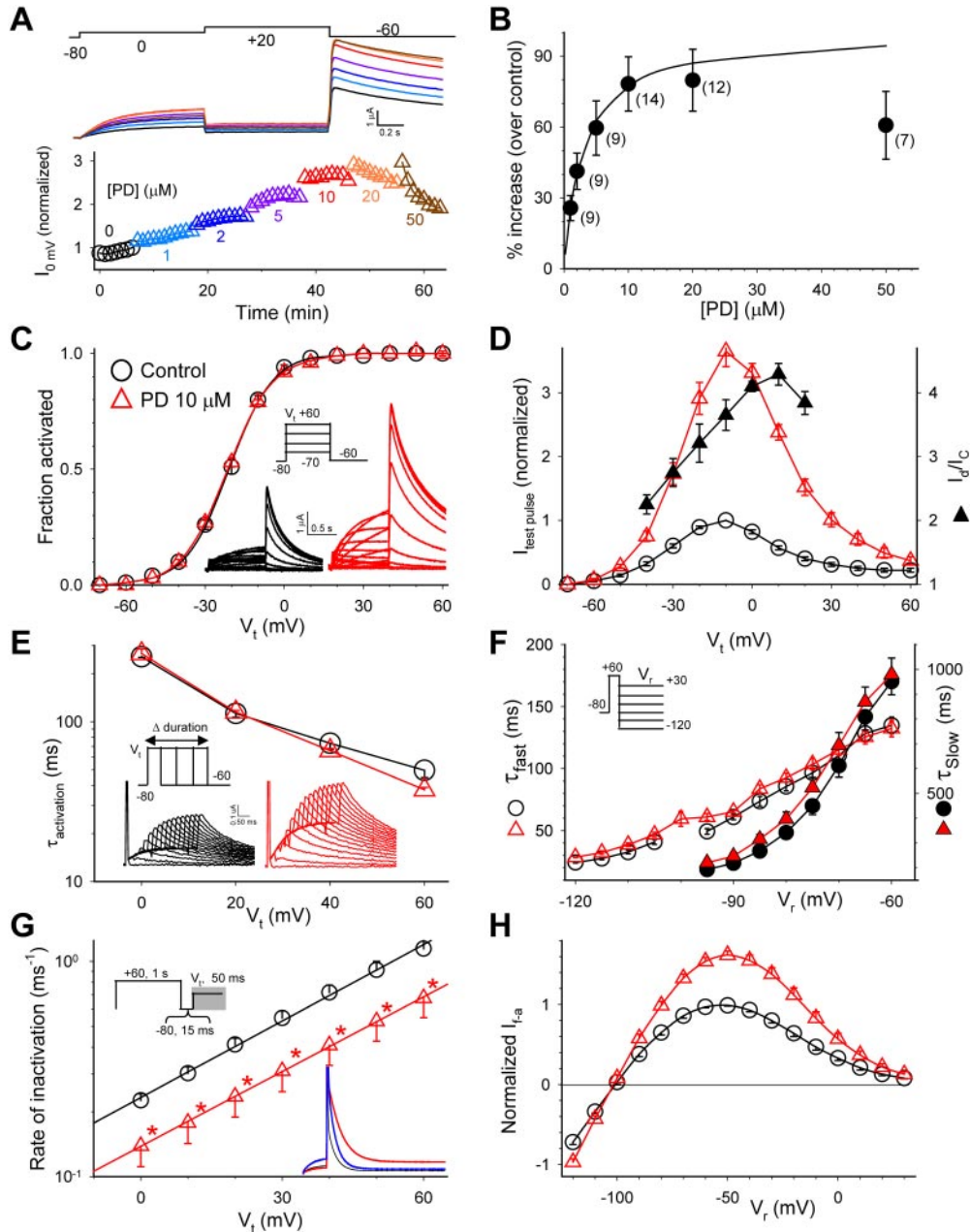
Fig. 1. Characterization of the effects of PD on the hERG channel expressed in oocytes. A , top, superimposed hERG current traces before (black) and after PD application (1, 2, 5, 10, 20, and 50 \mu\text{M} , traces shown in the same colors as those of symbols in the lower panel). The currents were elicited by the voltage clamp protocol diagrammed on top applied once every min. Bottom, time course of changes in hERG current amplitude from the same experiment. Current amplitudes were measured from the time-dependent current during the 0 mV step and normalized by the control current right before the start of PD application. B , concentration-response relationship. Numbers of measurements are shown in parentheses. The superimposed curve was calculated from the equation I_d/I_c = 1 + (A - 1)/(1 + K_d/[D]) , with A (-fold increase in current amplitude) = 2 and apparent dissociation constant ( K_d ) = 3 \mu\text{M} . In the following panels, data points and current traces recorded under the control conditions are shown in black, and those recorded in the presence of PD (10 \mu\text{M} ) are shown in red. C , PD did not shift the 1-s isochronal activation curve of hERG. Inset, voltage-clamp protocol and representative current traces. The relationship between V_t and peak amplitude of tail current ( I_{\text{tail}} ) was fit with a Boltzmann function: I_{\text{tail}} = I_{\text{max}}/[1 + \exp((V_{0.5} - V_t)/k)] , to estimate the maximal peak tail current amplitude ( I_{\text{max}} ), half-maximal activation voltage ( V_{0.5} ) and slope factor ( k ). I_{\text{tail}} was normalized by I_{\text{max}} ( I_{\text{tail}}/I_{\text{max}} = fraction activated) and plotted against V_t . D , PD increased hERG test pulse currents in a voltage-dependent manner. The voltage-clamp protocol was the same as that described for C. For each oocyte, amplitudes of time-dependent currents during 1-s test pulses to V_t were normalized by the control current at V_t -10 mV. The current ratios, I_d/I_c , are also plotted based on the right coordinate. E , PD did not alter the time course of hERG activation. Inset, "envelope" voltage clamp protocol and representative current traces. The rate of hERG activation was slower than inactivation. Thus the time course of activation could not be directly measured from the test pulse currents. Because the outward tail currents signified channels recovered from inactivation, the time course of growth of peak tail current amplitude after increasing durations of depolarizing pulses could be used to infer the time course of channel activation. The membrane voltage was stepped to V_t for durations varying from 5 to 1000 ms in 50-ms increments. The time course of growth of peak tail current amplitude was fit with a single exponential function to generate \tau_{\text{activation}} (plotted on a logarithmic scale so that the slope indicates the voltage-sensitivity of the underlying gating process). F , PD did not alter the time course of hERG deactivation. Inset, voltage-clamp protocol. Tail currents during 2- to 5-s step to V_r were fit with a double exponential function to generate the fast and slow time constants of deactivation ( \tau_{\text{fast}} and \tau_{\text{slow}} , right and left coordinates, respectively). In V_r range \leq -100 mV, channel deactivation was almost exclusively the fast component; thus \tau_{\text{slow}} values are not shown. G , PD modestly slowed the rate of hERG inactivation. Inset, triple-pulse voltage-clamp protocol and representative current traces during the third step (indicated by gray shade in the protocol diagram). The blue
