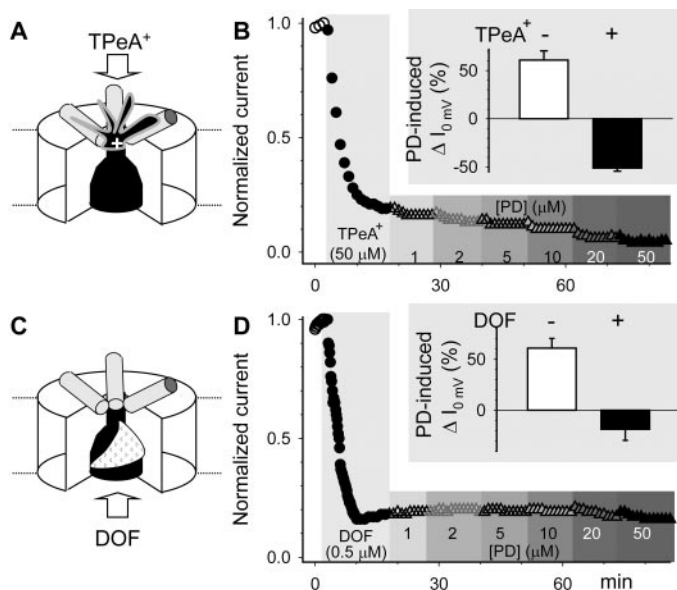
Fig. 9. An outer pore blocker, TPEA^+ , or an inner cavity blocker, dofetilide (DOF) prevented the activator effect of PD307243 on hERG. A, cartoon of a TPEA^+ ion binding to the outer pore entrance of hERG. B, time course of changes in hERG current amplitude before and after application of 50 \mu M TPEA^+ and after application of increasing concentrations of PD in the continuous presence of TPEA^+ . Current amplitudes were measured from time-dependent currents during 1-s step to 0 mV and normalized by control. Inset: summary of PD (20 \mu M )-induced changes in hERG current amplitude in the absence or presence of TPEA^+ . C and D, the format is the same as that in A and B. DOF binds from the intracellular side of the membrane to the inner cavity.
